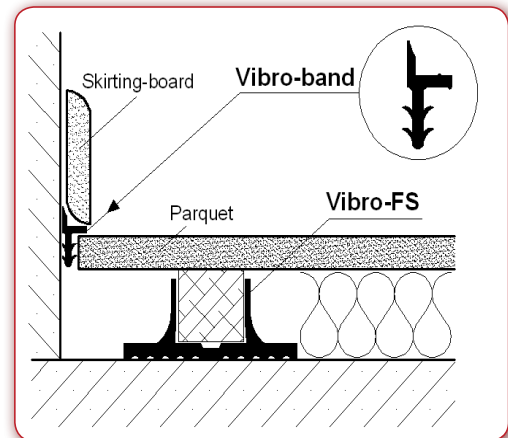
Section view of a parquet antivibration solution
