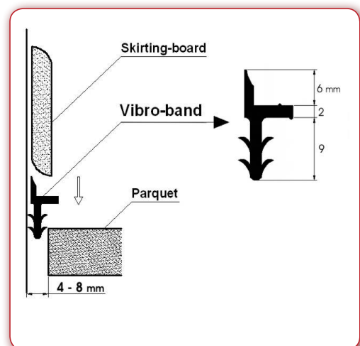
Section view of a parquet antivibration solution
